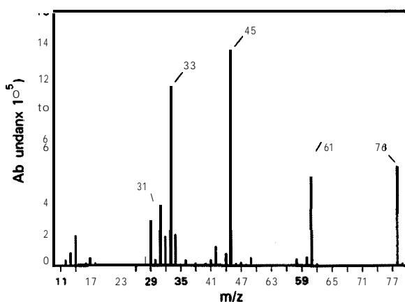
Fig. 1. Mass spectrum of monofluoroacetic acid. m/z 31 = fragment \text{FC}^+ ; m/z 33 = \text{FH}_2\text{C}^+ ; m/z 45 = \text{HO-C=O}^+ ; m/z 61 = \text{FH}_2\text{C-C=O}^+ ; m/z 78 = \text{M}^+ .
